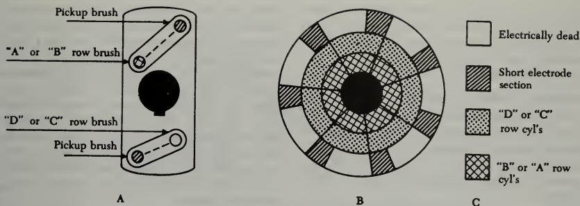
FIGURE 4-18. Brush-type distributor for a low-tension magneto system.
